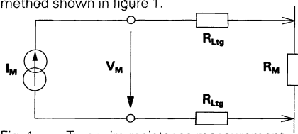
Fig. 1. Two-wire resistance measurement
